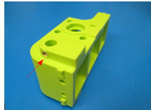
PP-GP0215 -- Z Lower Left v2.3
