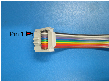
Pin 1 defined by arrow on connector 2x [PC-CN0010] Conn Socket IDC, 10POS DUAL
