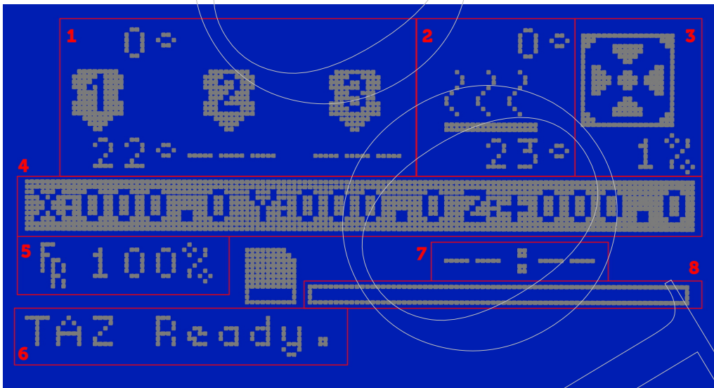
Figure 3.1: GLCD Info Screen
