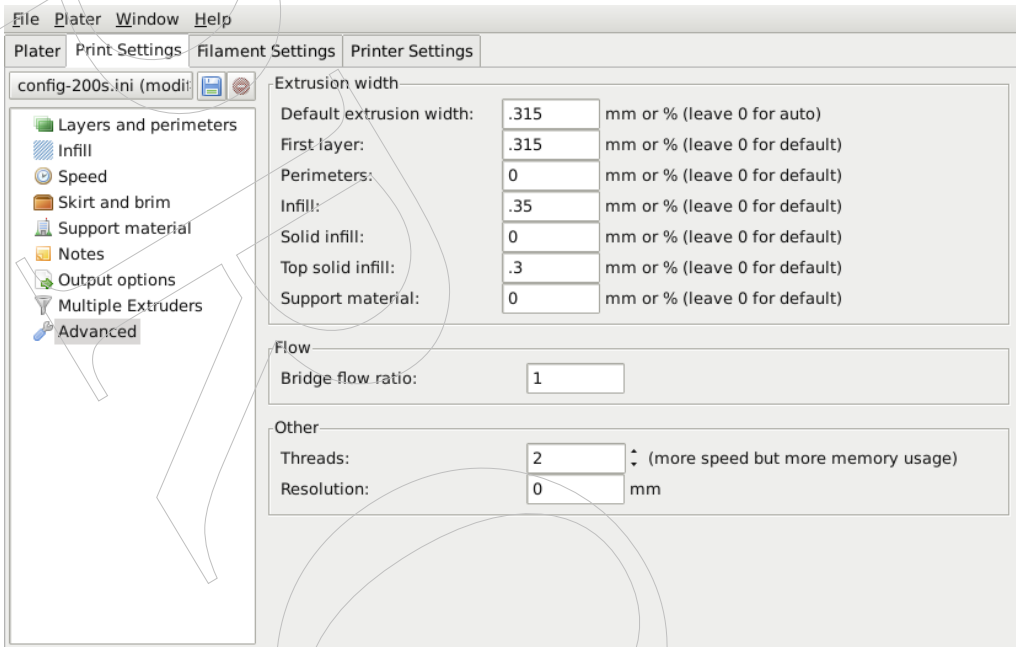
Figure 2.48: Extrusion widths options.
