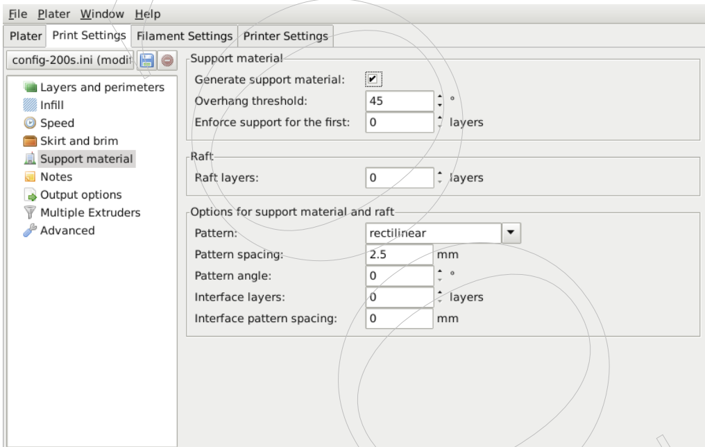
Figure 2.37: Support structure options.
