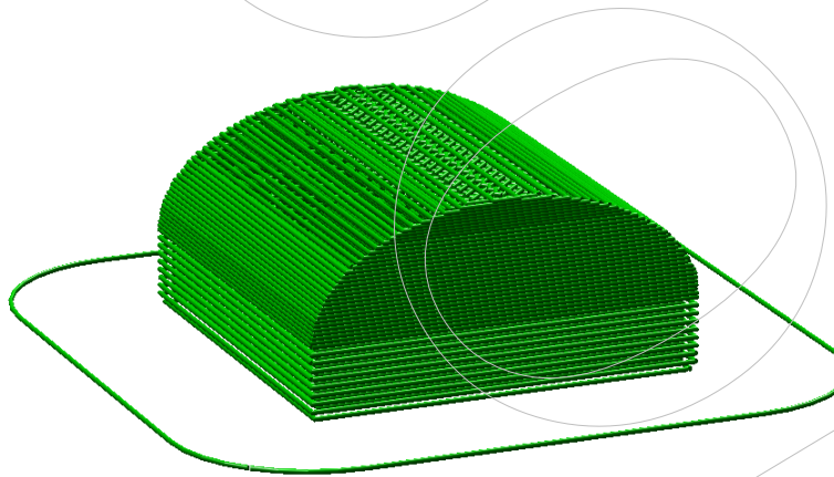
Figure 2.53: Example with variable layer height.
