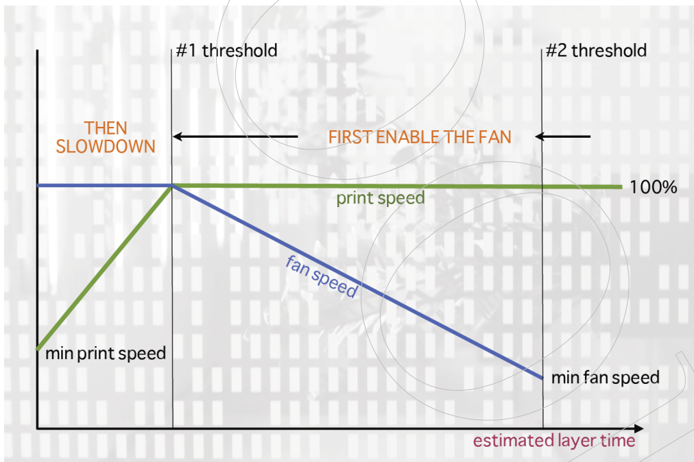
Figure 2.35: Cooling strategy.
