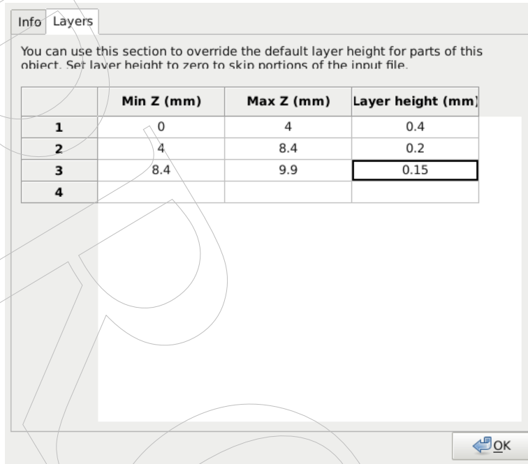
Figure 2.52: Variable layer height options - Layers.
